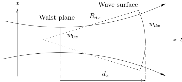
Figure 4. Gaussian beam parameters in the section of plane x-z . The direction of light propagation is z . The waist (transverse) radius is w_{0x} . The principal curvature radius of the wave surface at a distance d_x is R_{dx} , and the transverse beam radius (along x ) on this surface is w_{dx} . An equivalent diagram can be drawn in the orthogonal y-z section, with parameters w_{0y} , d_y , R_{dy} and w_{dy} . The Gaussian beam is astigmatic if w_{0x} \neq w_{0y} or if d_x \neq d_y ; then R_{dx} \neq R_{dy} and w_{dx} \neq w_{dy} . The Gaussian beam is cylindrical if w_{0x} = w_{0y} and d_x = d_y ; then R_{dx} = R_{dy} and w_{dx} = w_{dy} , and indices x and y are dropped.
