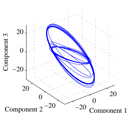
Figure 1: Elliptical trajectory
