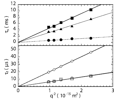
FIG. 5. Variation of both slow ( \tau_s , closed symbols) and fast ( \tau_f , open symbols) characteristic times as a function of q^{-2} for \phi_d = 0.022 ( \diamond ), 0.157 ( \bullet , \circ ), 0.265 ( \blacktriangle , \triangle ), and 0.283 ( \blacksquare , \square ).
