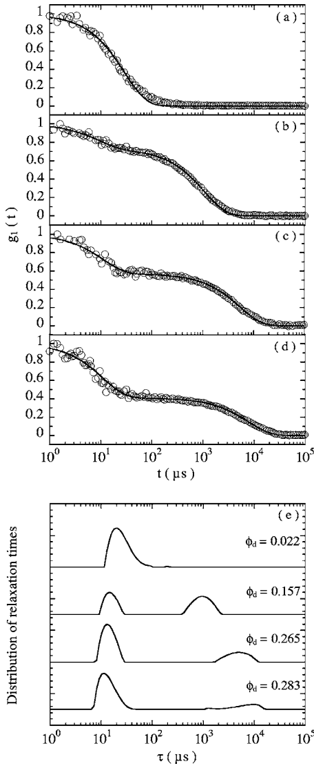
FIG. 4. Normalized autocorrelation functions obtained at an angle of 90^\circ for (a) \phi_d=0.022 , (b) 0.157, (c) 0.265, and (d) 0.283. For (b), (c), and (d) the continuous lines are the best fits obtained for the data with the sum of two exponentials (b) g_1(t) = 0.27 \exp(-t/9) + 0.73 \exp(-t/1057) , (c) g_1(t) = 0.43 \exp(-t/11) + 0.57 \exp(-t/5358) , and (d) g_1(t) = 0.59 \exp(-t/11) + 0.41 \exp(-t/7680) . For (a) The continuous line is the best fit obtained with a monoexponential, namely, g_1 = \exp(-t/29) , where t is the given in \mu\text{s} . The temperature is T=25^\circ\text{C} . (e) Distribution of the relaxation times obtained by an inverse Laplace transformation of the autocorrelation functions presented in Figs. 4(a)–4(d).
