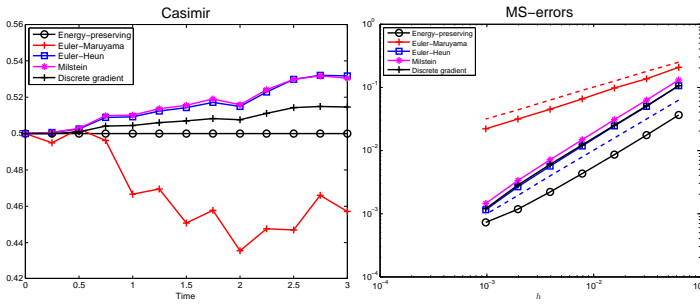
Fig. 4.3 Computed Casimirs along the numerical solutions of a stochastic rigid body (left). The right plot displays the mean-square order of the schemes: the reference solution is computed using Milstein's method with h_{\text{exact}} = 2^{-12} and M = 1000 samples were used for the expectations. The dashed lines have slopes 1/2 and 1 .
