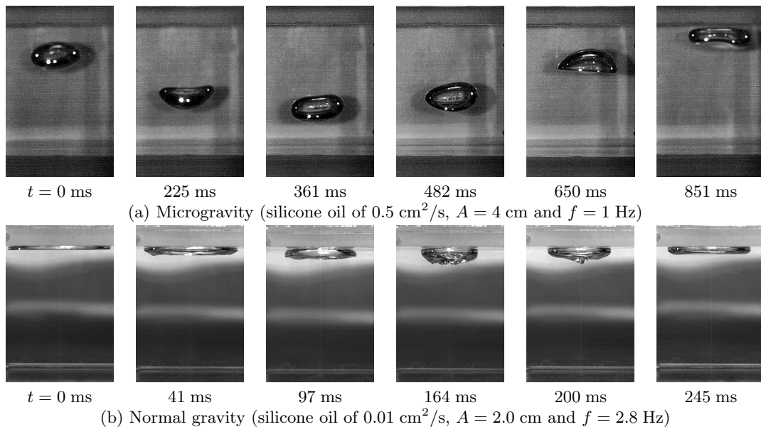
Fig. 2. Side views of bubble motion under oscillatory acceleration field.
