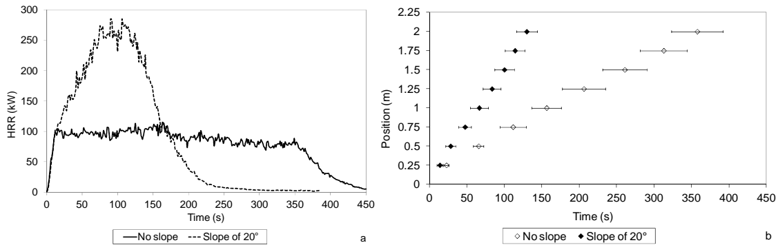
FIG. 3 –a) Heat release rate b) Mean position of the head of the fire front
