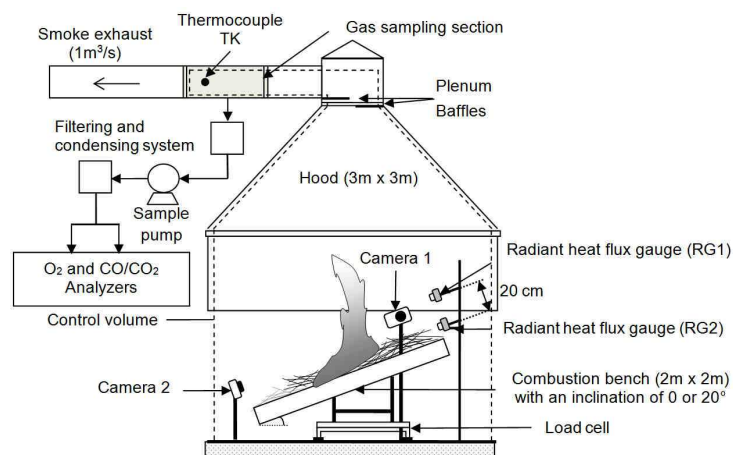
FIG. 1 – Experimental device for the fire spread study
