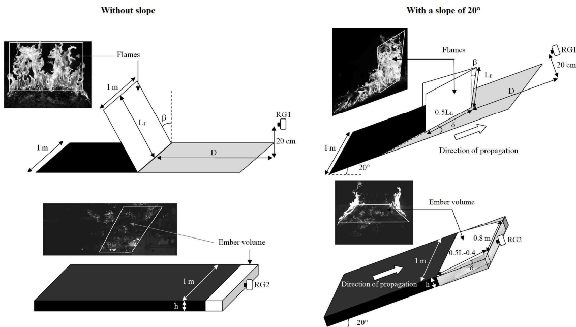
FIG. 4 – Diagrams describing the modeling of the fire front for the calculation of the view factors
