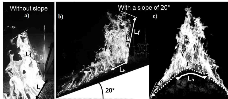
FIG. 2 – Geometric descriptors of the fire front a) no-slope lateral view b) slope lateral view c) slope rear view
