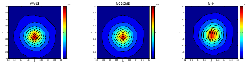
Figure 4: Contour plots of the fluence rate estimates in the plane x = -0.04 for WANG, MC-SOME and MH.
