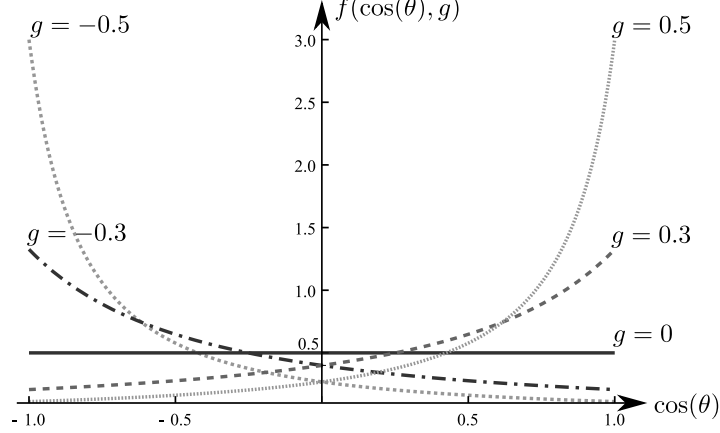
Figure 1: Density function of \cos(\theta) = \langle \omega, \hat{\omega} \rangle when \hat{\omega} is scattered according to the Henyey-Greenstein function f_{HG}(\omega, \cdot) for several values of the anisotropy parameter g .
