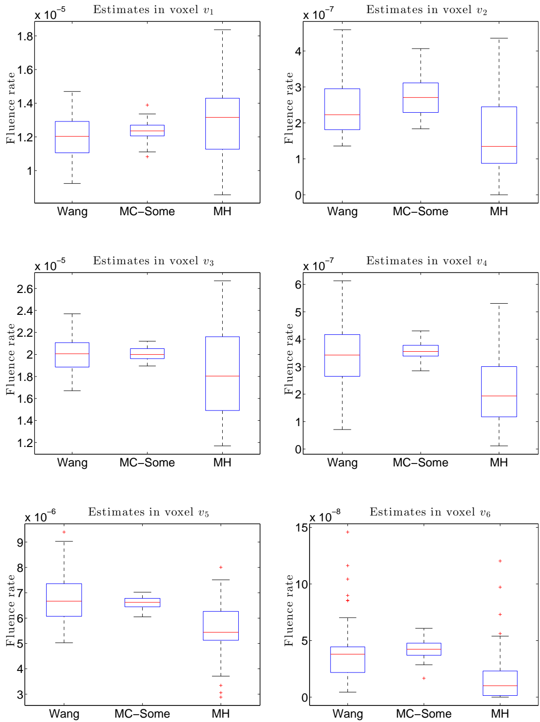
Figure 7: Boxplots of 50 fluence rate estimates in the voxels (v_i)_{i=1,\dots,6} with WANG, MC-SOME and MH.
