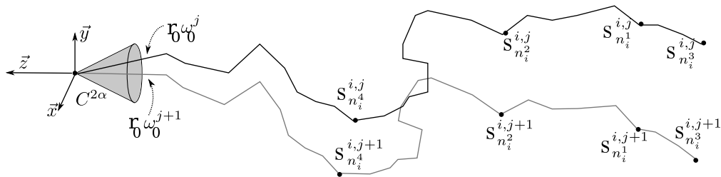
Figure 2: Description of MC-SOME method. In this example, the grey path is a rotation of the black one with respect to its initial direction \omega_0^{j+1} and M = 4 .
