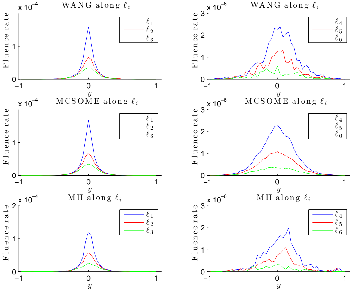
Figure 6: Fluence rate estimates along the lines (\ell_i)_{i=1,\dots,6} with WANG, MC-SOME and MH.
