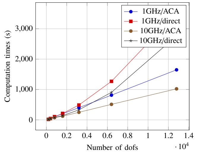
Figure 3: Computation times.
