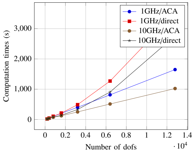
Figure 3: Computation times.
