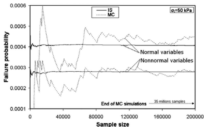
Fig. 10. Failure probability versus the number of samples for correlated variables as given by IS and MC
