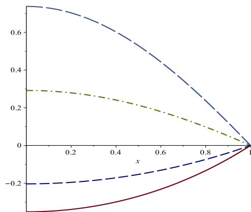
FIGURE 4. A few minimizers as given by formula (4.9), for \alpha = 2, 1, -1, -2 (from bottom to top).
