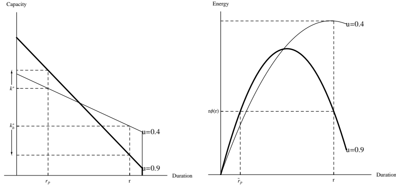
(a) Two load duration curves and (b) The marginal risk from investment T.k with the two load duration curves, and the threshold \tilde{r}_p of Corollary 1
