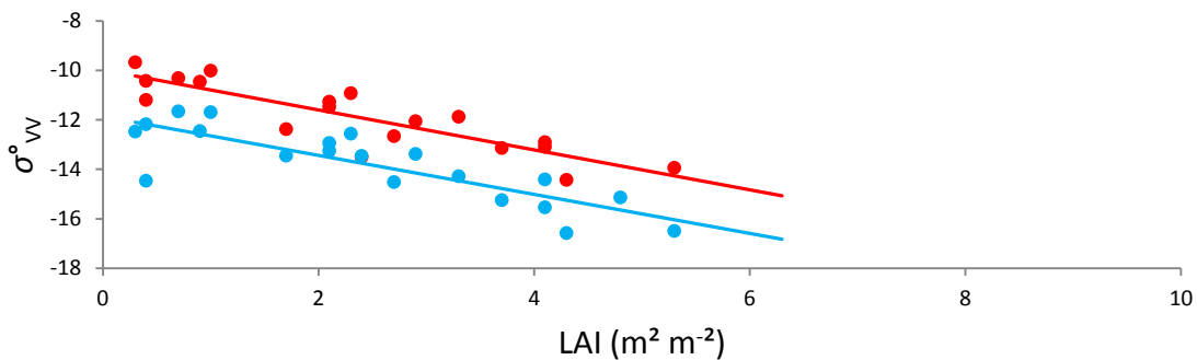
Figure 2 - VV-polarization backscattering values ( \sigma^{\circ}_{VV} ) of TSX (red dots), at an incidence angle of 35° and CSK (blue dots) at 45°, versus LAI of barley and wheat on 16 April 2012. Lines represent the regression equations and refer to different datasets (red: TSX; blue: CSK).
