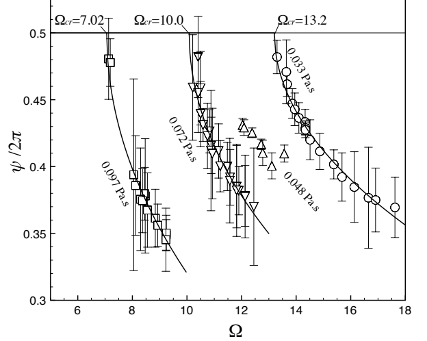
(a) Normalized divergence angles showing a bifurcation from an alternate pattern ( \psi = \pi )
