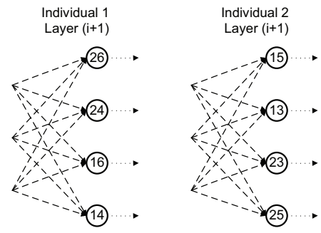
Figure 6: Phase 4b: the offspring generated by the crossover operator.
