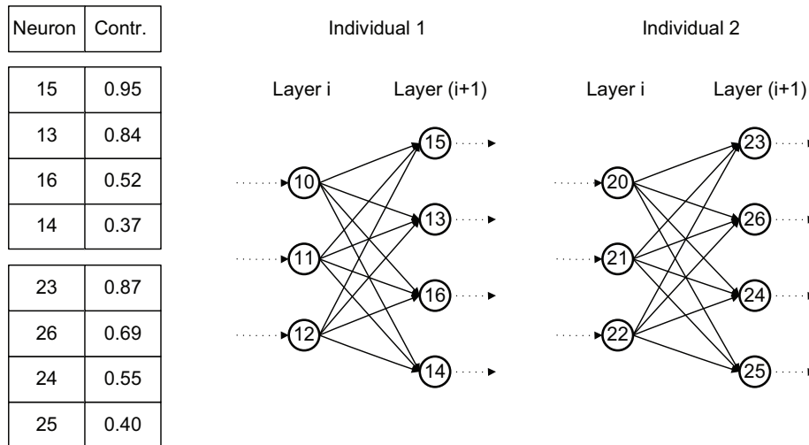
Figure 3: Phase 2: the contribution of each neuron of layer i + 1 of the two parents is computed, then the neurons of the (i + 1) th layer of the two parents are reordered according to their contribution. An example of the neuron contributions is shown in the table.
