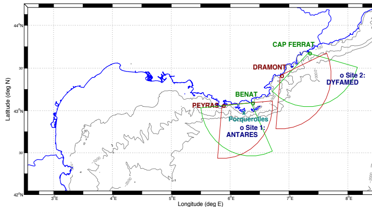
Fig. 1. Map of the HFSWR sites: #1 ANTARES-TOULON, #2 DYFAMED/Ligure. On site 1 ANTARES : the configuration is one monostatic radar at Cap Sicié (Peyras), one standalone transmitter on Porquerolles island, and its receiver at Cap Bénat (18 km far away). On site 2 DYFAMED : it will be covered with two radar seasons, one located at Cap Ferrat, and the other at Dramont. The arc of circles show the approximate radar coverage area of each system
