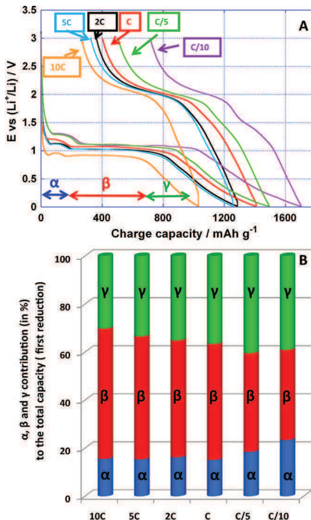
Fig. 2. (A) Plot of potential versus charge capacity profile for \text{Co}_3\text{O}_4 composite electrodes upon the first cycle at different C rates and (B) plot of the charge capacity percentage for each process (i.e. insertion \alpha ; conversion \beta and extra capa \gamma ) with respect to the total capacity achieved upon the first reduction.
