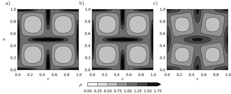
FIG. 4.5. Snapshots of the density distribution at time t=0.33 for Stokes number St = 0.9St_c : 2 nd order Bouchut scheme (a), 2 nd order pressureless relaxation scheme (b) and 2 nd order relaxation scheme with pressure (c) (200 nodes, CFL=0.5 ).
