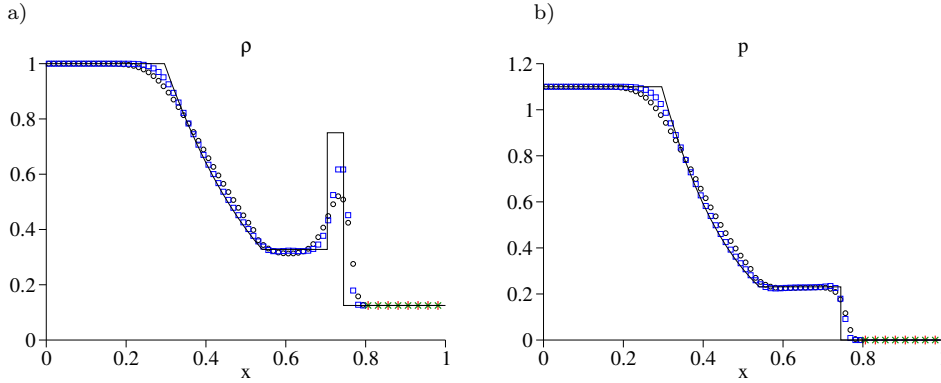
FIG. 4.2. Profiles of density (a) and pressure (b) for the hybrid relaxation scheme in Sod numerical test at time t = 0.1644 : 1 st order relaxation scheme (pressure region: \circ , pressureless region: + ), 2 nd order relaxation scheme (pressure region: \square , pressureless region: \times ) (80 nodes, CFL = 0.5).
