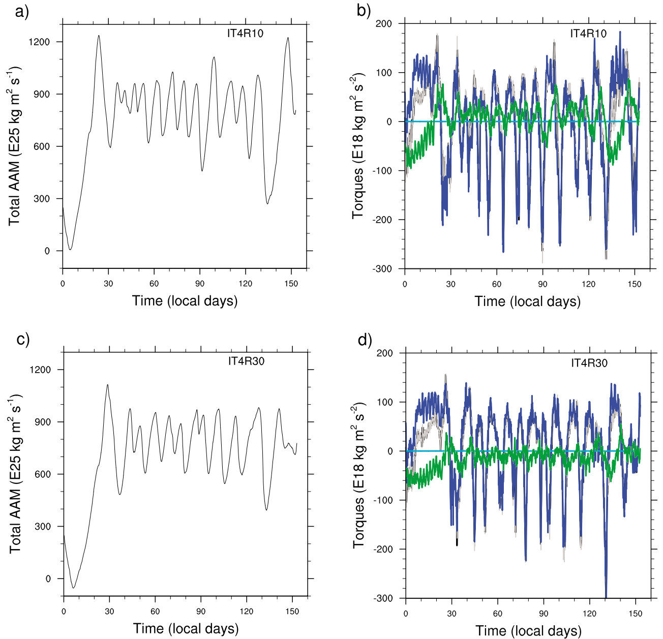
Figure 4. Same as Figure 3, but with a reduced coefficient for the 4th-order divergence damping. (a, b) IT4R10 and (c, d) IT4R30. Torques color scheme: black, dM_e/dt ; gray, \Sigma ; light blue, F ; blue, T ; green, \epsilon^* .
