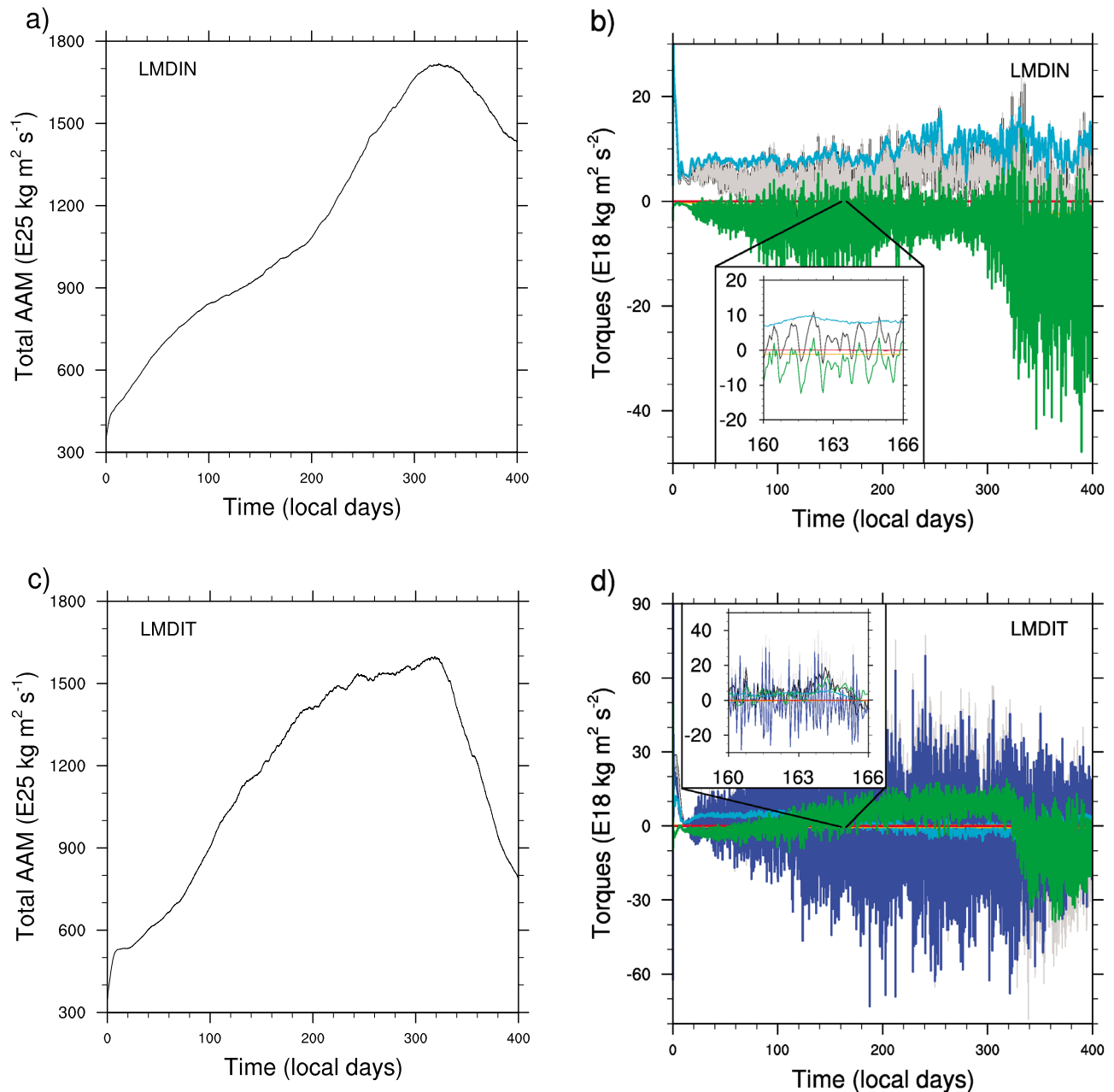
Figure 1. LMD idealized physics simulations: (a, b) without topography (LMDIN), (c, d) with topography (LMDIT); (Figures 1a and 1c) M . The color scheme for the torques is: black, dM_r/dt (computed as a temporal centered difference from M_r ); gray, \Sigma = F + D_y ; light blue, surface friction F ; blue, mountain torque T ; orange, horizontal dissipation D ; red, sponge layer S ; green, residual from dynamics \epsilon .
