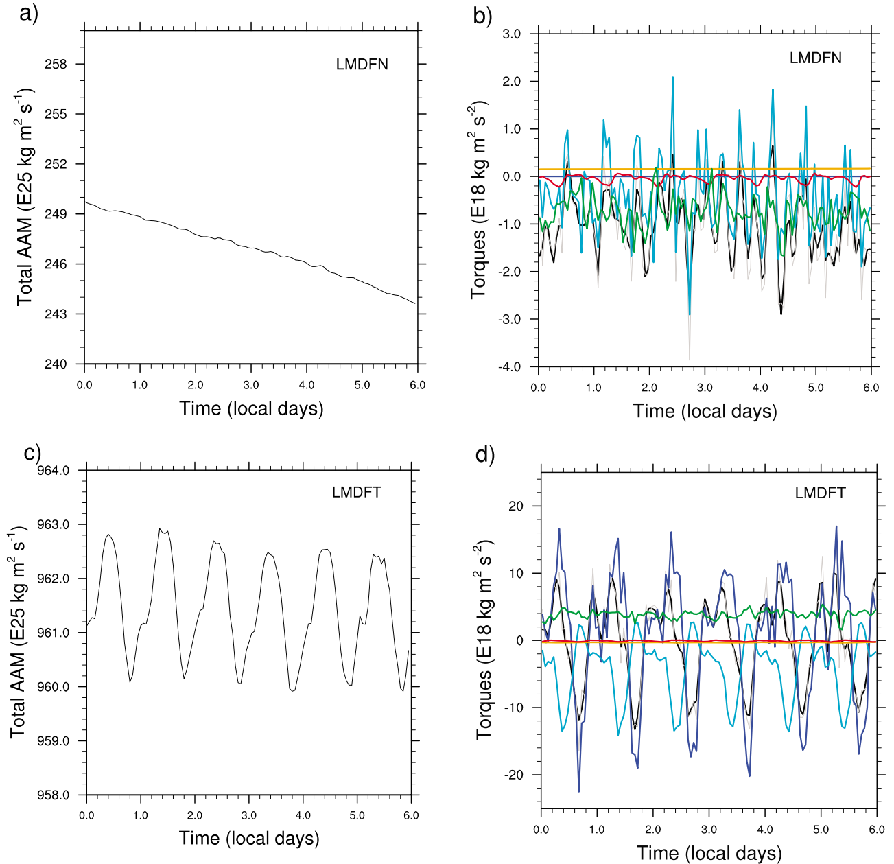
Figure 2. LMD full physics simulations: (a, b) without topography (LMDFN), (c, d) with topography (LMDFT); (Figures 2a and 2c) M . Torques color scheme: black, dM_e/dt ; gray, \Sigma ; light blue, F ; blue, T ; orange, D ; red, S ; green, \epsilon . For clarity purposes, only 6 Venus days taken from our simulations are plotted.
