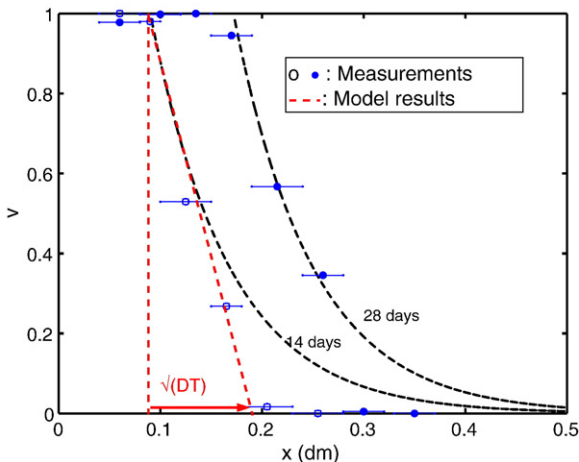
Fig. 12. v profiles for the P45 cement paste after 14 and 28 days of accelerated exposure. Experimental and simulated profiles.
