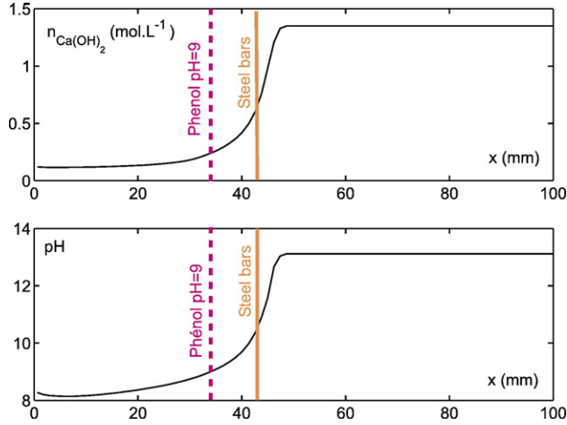
Fig. 1. Schematic sketches of \text{Ca(OH)}_2 content and pH-profiles in the concrete cover when the concrete has been carbonated to a certain depth.
