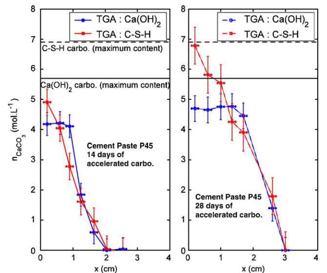
Fig. 6. \text{Ca(OH)}_2 and C–S–H carbonation profiles after a 14-day and a 28-day accelerated carbonation test of the cement paste P45.
