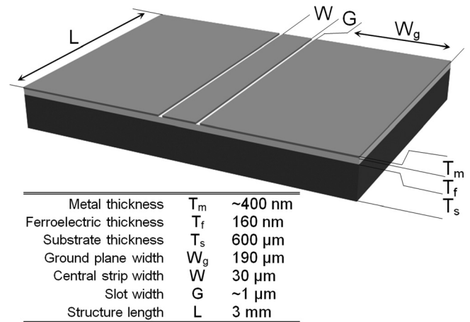
FIG. 1. Schematic view of Non-Linear Co-Planar Waveguide (NL-CPW).
