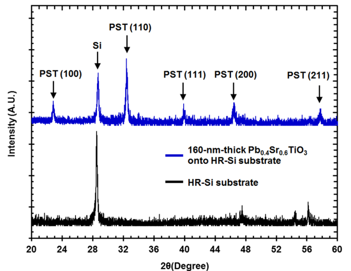
FIG. 3. X-ray diffraction patterns of PST film deposited on HR-Si substrate with a post annealing temperature of 650 °C. Black line: HR-Si substrate alone. Blue line: 160-nm-thick PST onto HR-Si substrate.
