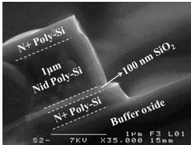
Figure 2: SEM of the optimized sidewall profile, which enables the active layer, the gate oxide layer, and the Al layer depositions on it. It remains, however, a small recess at the level of the \text{SiO}_2 insulating layer due to the etching selectivity difference.
