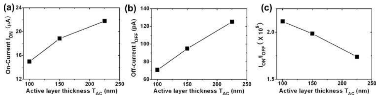
Figure 5: (a) On-current I_{ON} , (b) off-current I_{OFF} , and (c) I_{ON}/I_{OFF} relationships with different active layer thicknesses T_{AC} . I_{ON} and I_{OFF} increases with T_{AC} , while I_{ON}/I_{OFF} reduces when increasing T_{AC} .
