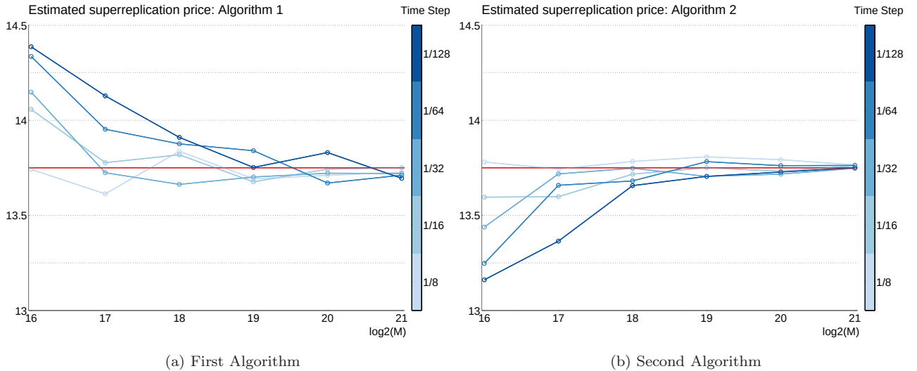
Figure 3.7: Price of Outperformer Option ( \rho = -0.5 )
