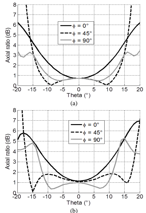
Fig. 9. Angular variation of axial ratio @ 3.90 GHz. (a) Simulation, and (b) measurements.
