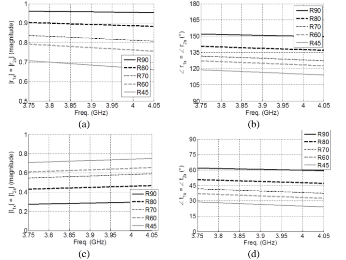
Fig. 10. HFSS simulation results for FSS with reflectivity values ranging between 45% and 90%. Reflection coefficient in magnitude (a) and phase (b). Transmission coefficient in magnitude (c) and phase (d). Both FSS are assumed identical.
