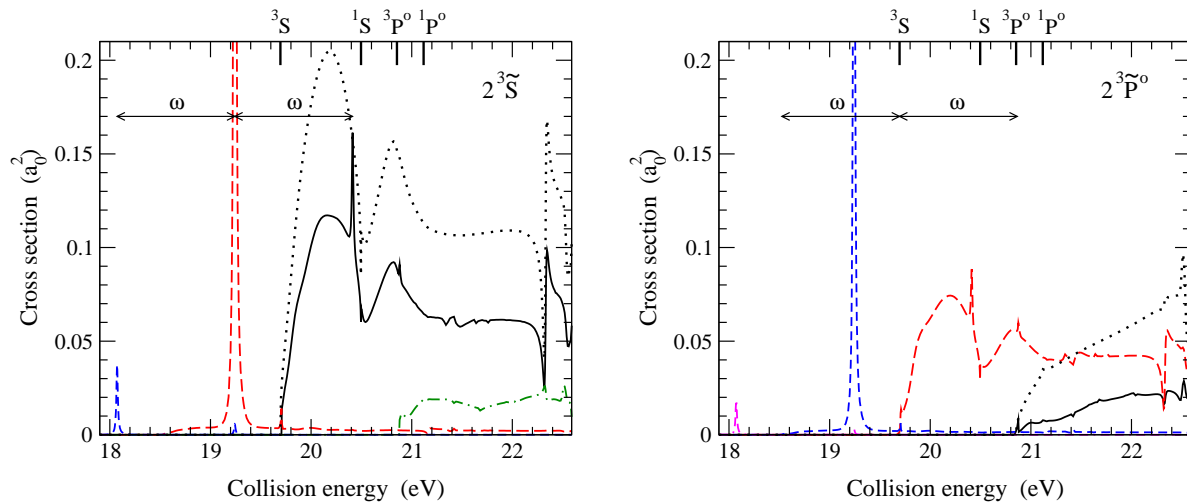
Figure 1. Cross sections for simultaneous electron-photon excitation of helium into the field-dressed 2 {}^3\tilde{S} and 2 {}^3\tilde{P}^\circ ( M_f = 0 ) states, in the presence of a Nd:YAG laser field of intensity 10^{10} \text{ W cm}^{-2} . The electron is incident parallel to the laser polarization axis. —, no net exchange of photons; - - -, net absorption of one photon; - - - -, net absorption of two photons; - · · -, net absorption of three photons (giving rise to the small peak close to 18.1 eV; right panel only); - · -, net emission of one photon (left panel only). The dotted lines are the corresponding field-free cross sections for excitation into the 2 {}^3S and 2 {}^3P^\circ states. The field-free thresholds are indicated along the upper edge of the graphs. In the left panel, the horizontal arrows of length \omega indicate the replication of the main \text{He}^-(1s2s^2 {}^2S) resonance by absorption or emission of one photon. In the right panel, the arrows indicate the similar replication of the 2 {}^3S and 2 {}^3P^\circ thresholds.
