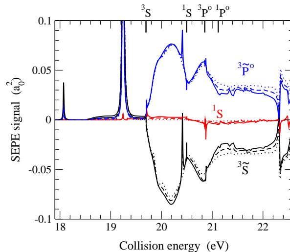
Figure 6. SEPE signals (difference between the laser-assisted and field-free cross sections) for excitation into the 2^3\tilde{S} , 2^1S and 2^3\tilde{P}^0(M_f = 0, \pm 1) dressed states, for different values of the angle \theta_{in} between the incident electron momentum \mathbf{k}_i and the laser polarization axis. —, \theta_{in} = 0^\circ ; ---, \theta_{in} = 45^\circ ; \cdots , \theta_{in} = 90^\circ .
