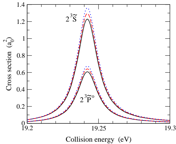
Figure 5. The \text{He}^-(1s2s^2\tilde{S}) resonance in the total cross sections (summed over the number of photons exchanged) for SEPE into the 2^3\tilde{S} and 2^3\tilde{P}^o(M_f = 0) dressed states, for different values of the angle \theta_{\text{in}} between the incident electron momentum \mathbf{k}_i and the laser polarization axis. —, \theta_{\text{in}} = 0^\circ ; - - -, \theta_{\text{in}} = 45^\circ ; ·····, \theta_{\text{in}} = 90^\circ . In both cases, the maximum increases by approximately 11% as \theta_{\text{in}} is varied from 0^\circ to 90^\circ , while their ratio remains close to 2.
