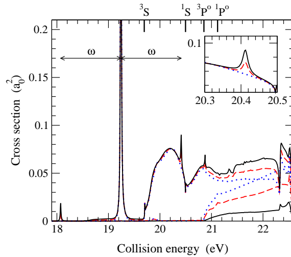
Figure 4. Total cross sections summed over the number of photons exchanged for SEPE into the 2^3\tilde{P}^o(M_f=0) (upper curves) and the 2^3\tilde{P}^o(M_f = \pm 1) (lower curves starting at the 2^3\tilde{P}^o threshold) states as a function of collision energy for different angles \theta_{\text{in}} between the incident electron momentum \mathbf{k}_i and the laser polarization axis. —, \theta_{\text{in}} = 0^\circ ; - - -, \theta_{\text{in}} = 45^\circ ; ·····, \theta_{\text{in}} = 90^\circ . The resonances at one photon energy below and above the \text{He}^-(1s2s^2\tilde{S}) resonance are suppressed for \theta_{\text{in}} = 90^\circ . Above the 2^3\tilde{P}^o threshold, the cross sections are more sensitive to \theta_{\text{in}} than those for SEPE into the 2^3\tilde{S} dressed state, in particular for M_f = \pm 1 .
