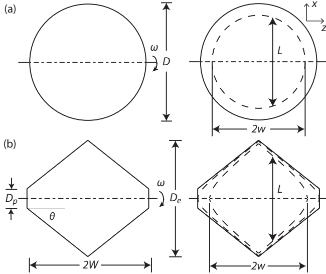
FIG. 9. Top views of (a) spherical tumbler of diameter, D , and (b) truncated double cone tumbler of width, 2W , equator diameter, D_e , and pole diameter, D_p . Rotation is about the z -axis, which is also the axis of symmetry for the double cone tumbler. (Left column) Bed cross sections at fill fraction f = 50\% . (Right column) Sketches of the flowing layer surface (dashed curves) in the xz -plane for f \neq 50\% with flowing layer width, 2w , along the axis of rotation. The flowing layer length, L , varies axially for both spherical and conical tumblers. 2W is the axial width of the tumbler while 2w is the axial distance that the free surface extends in the tumbler, which may be less than the width of the tumbler depending of the fill level.
