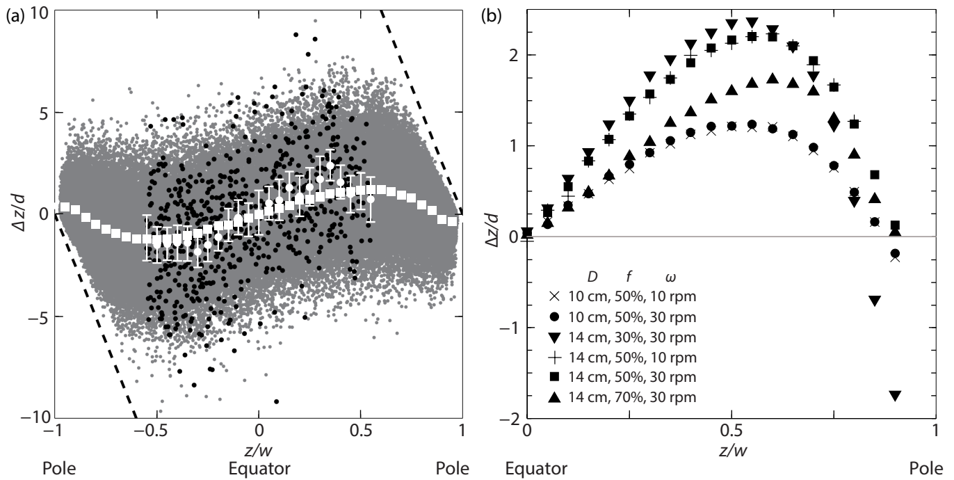
FIG. 8. Non-dimensional axial surface drift per pass \Delta z/d vs. normalized axial position z/w in a spherical tumbler with d = 2 -mm particles. (a) \Delta z/d from experiment (black points) and simulation (gray points) are similar. Mean axial drift with 95% confidence interval error bars for experiment (white circles) and for simulation (white squares) match within uncertainty (error bars for simulation are smaller than the symbols). Axial distance to the poles (dashed lines) bounds the axial displacement. f = 50\% and \omega = 10 rpm. (b) Mean axial surface drift in spherical tumbler simulations increases with D . w is the half width of the free surface.
