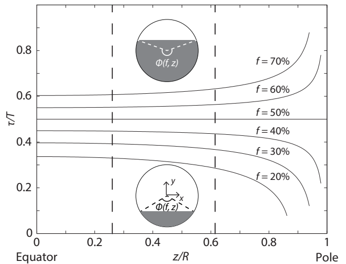
FIG. 3. Calculated axial variation of normalized solid body rotation time, \tau/T , vs. normalized axial position, z/R , for 20\% \leq f \leq 70\% in a spherical tumbler. Curves extend from the equator to the maximum axial position of the free surface. The region between vertical dashed lines represents the initial position of the tracer band ( 0.257 < z/R < 0.614 ) in experiments and simulations.
