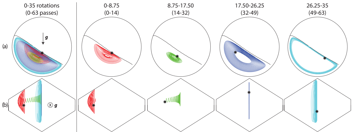
FIG. 10. (Color Online) Mean particle trajectory for a double cone tumbler simulation: (a) side view ( xy plane) and (b) top view (parallel to \vec{g} ). Trajectory is shown for 35 rotations (63 flowing layer passes) in its entirety (first column) and in 8.75 tumbler rotation segments with 2W = 15 cm, D_p = 2.5 cm, D_e = 12 cm, and \theta = 26.6^\circ . Tumbler rotations are given above each column with flowing layer passes in parentheses. Similar to the spherical tumbler (Fig. 7), straight portions of the trajectory in (b) correspond to solid body rotation while curved portions correspond to flow [43]. The free surface is indicated by the black curves in (a). The trajectory starts 0.6 mm below the surface and directly below the axis of rotation at z/W = 0.53 (asterisk), advances towards the pole through the top of the flowing layer, and returns to the equator through the bottom of the flowing layer. f = 30\% , d = 2 mm, and \omega = 30 rpm.
