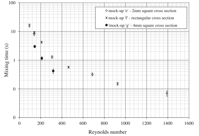
Fig. 21. Mixing times vs. Reynolds number according to the channel design.
