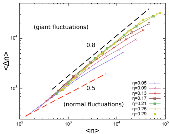
FIG. 3: Number fluctuations of SA2407 cells - at low packing fractions \eta , number fluctuations \Delta n are consistent to what is expected for normal fluctuations. For large values of \eta , i.e., for \eta \geq \eta_c , number fluctuations are giant, with a critical exponent 0.85 \pm 0.05 .
