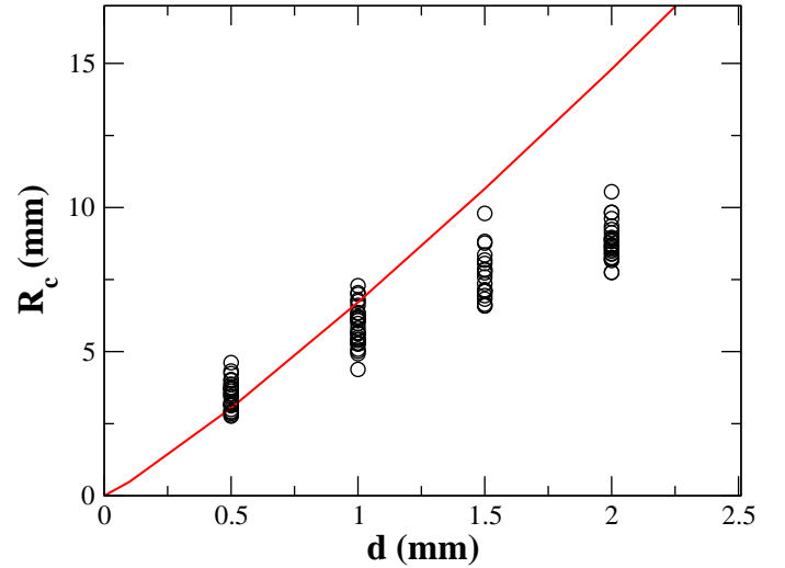
FIG. 9: Critical radius R_c versus the spacing d . Each point corresponds to one experiment. The red line holds for the numerical prediction using Eqs. (15-19)
