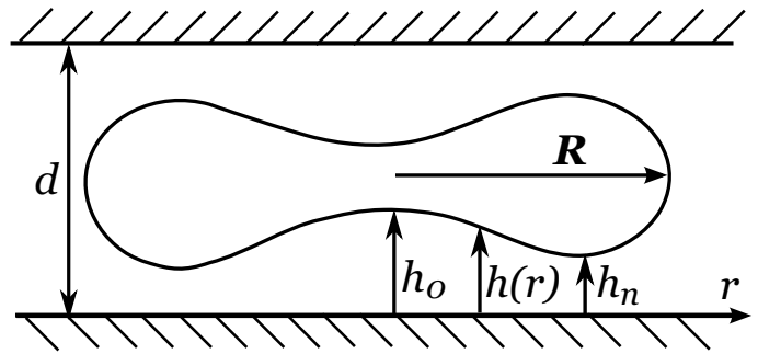
FIG. 6: sketch of a vertical cut of a drop. h_0 , h_n and R are shown.
