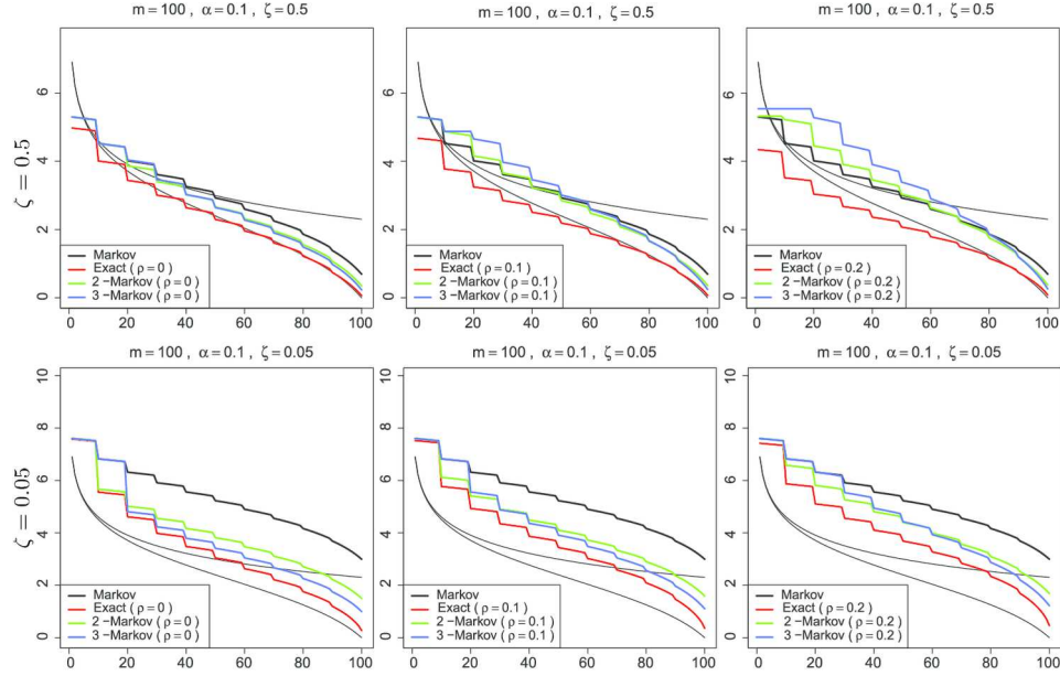
FIG. 3. Plot of -\log(\tilde{\tau}_\ell) in function of \ell \in \{1, \dots, m\} , for k -FWE-based critical values obtained with several types of bounding devices and assuming (Gauss- \rho -equi). For comparison, the solid thin black line corresponds either to the BH critical values -\log(\alpha\ell/m) (nonadaptive) or the AORC critical values -\log(\alpha\ell/(m - (1 - \alpha)\ell)) defined in Finner, Dickhaus and Roters (2009) (adaptive).
