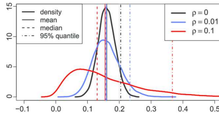
FIG. 1. Fitted density of the false discovery proportion of the BH procedure when increasing the dependence. m = 1000 , m_0 = 800 (number of true null hypotheses), 10^4 simulations, Gaussian one-sided equicorrelated model.
