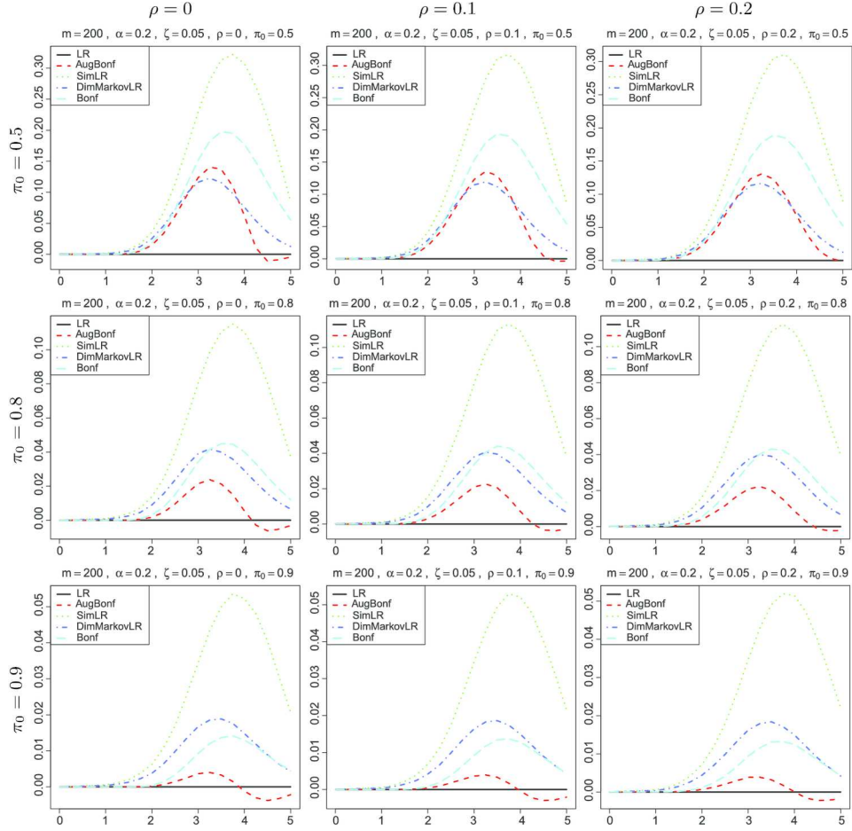
FIG. 4. Relative FNR to the Lehmann–Romano procedure in function of \beta ; see text and Table 1. Procedures not using the value of \rho .
