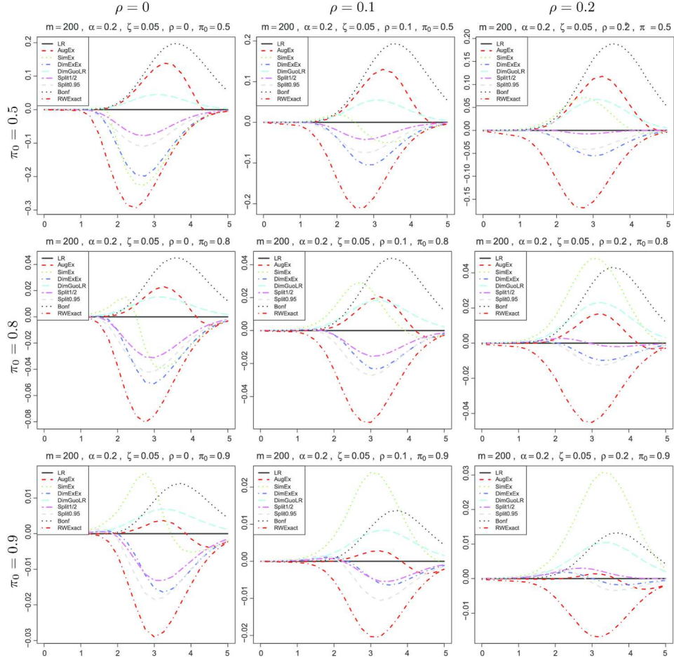
FIG. 5. Relative FNR to the Lehmann–Romano procedure in function of \beta ; see text and Table 1. Procedures using the value of \rho (except [LR] and [Bonf]).
