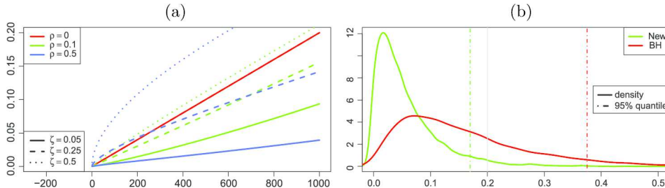
FIG. 2. (a) plot of the critical values (2) in function of l . (b) same as Figure 1 but only for \rho = 0.1 and by adding the new step-up procedure using (2). m = 1000 , \alpha = 0.2 , Gaussian one-sided \rho -equi-correlated model.
