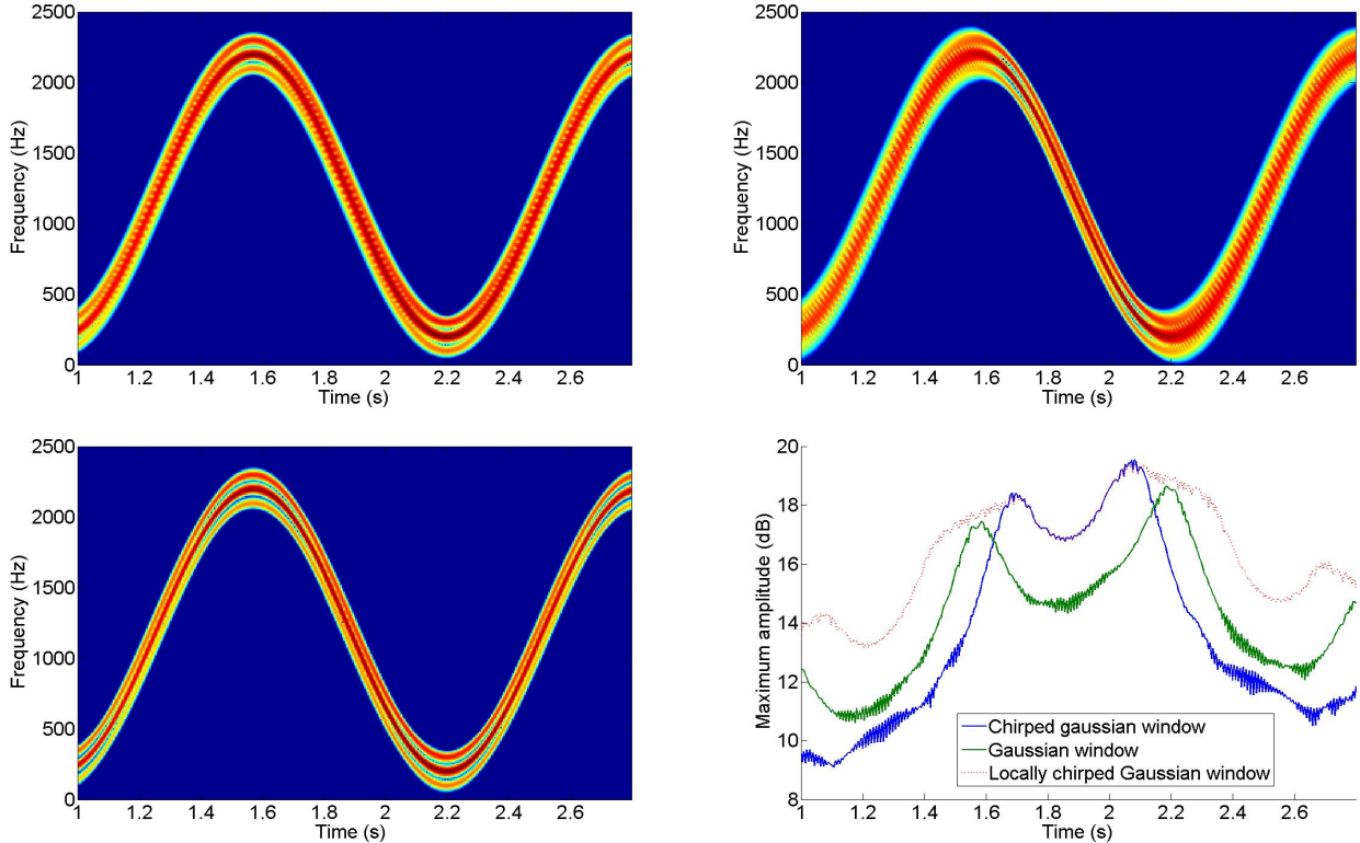
Figure 3: Spectrogram of an oscillating chirp in the TF plane with three different windows. Top left: Gaussian window. Top right: Optimal window for time interval [1.6, 2] . Bottom left: Optimal window evolving with time. Bottom right: Evolution in time of the maximum over frequencies of the spectrogram coefficients, for the 3 windows.
