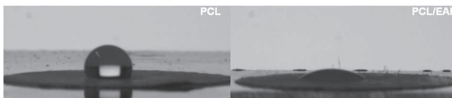
Fig. 2. Contact angle images of two of the scaffolds investigated.
