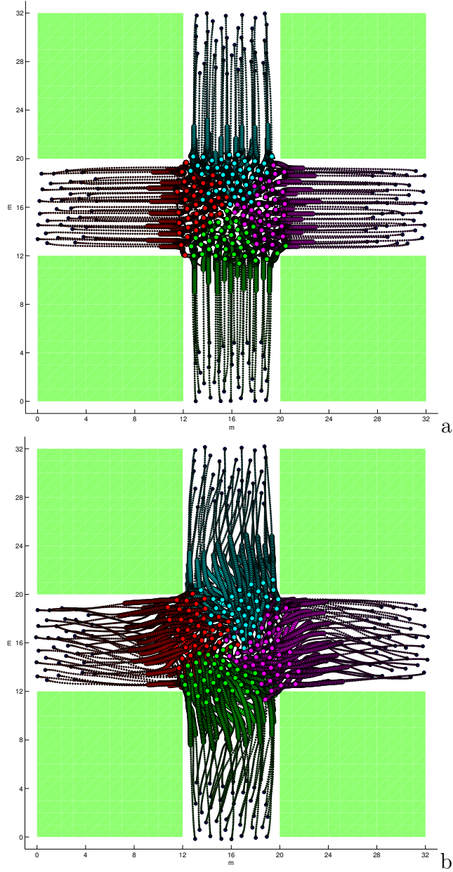
Figure 8: Trajectories of pedestrians for a duration of 20 seconds. The position of the individuals between the t = 12 s and t = 17 s are highlighted: (a) output of the crowd simulation, (b) output of the crowd optimization.
