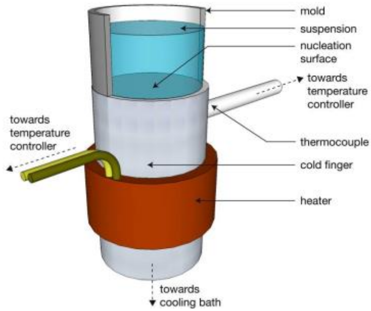
Figure 1: Experimental setup
