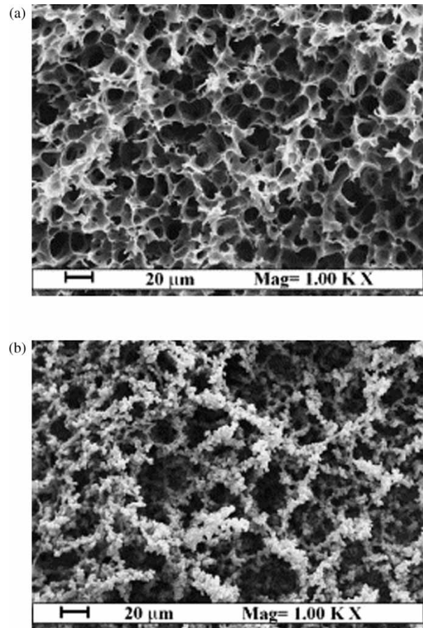
Figure 7. Membrane section T = 65^{\circ}\text{C} , P = 100 bar: (a) 20% (w/w); (b) 5% (w/w). Reprinted from Reverchon and Cardea (2004). Copyright 2004 with permission from Elsevier.
