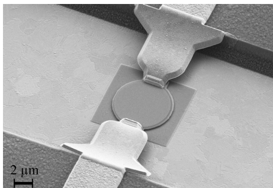
FIG. 1. SEM micrograph of a LT-GaAs metallic-mirror-based resonant photoconductor linked to two 50- \Omega thin film microstrip lines.
