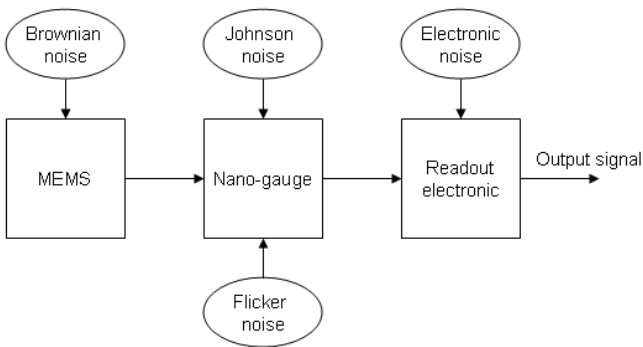
Fig. 3. Electro-mechanical noises in transduction chain.
