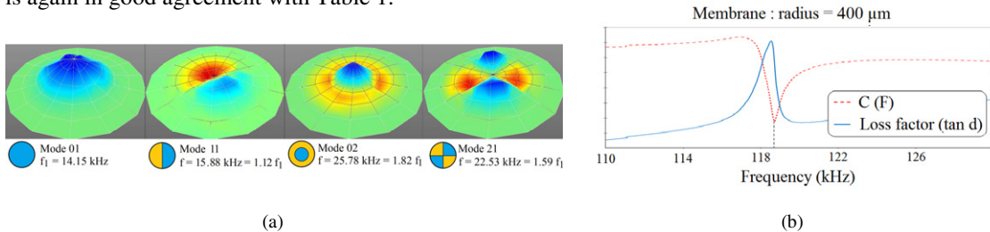
Fig. 3. (a) The first four modal deformations of the 2500 µm radius speaklet; (b) Impedancemeter measurement: capacity and loss factor versus frequency of the 400 µm radius speaklet
