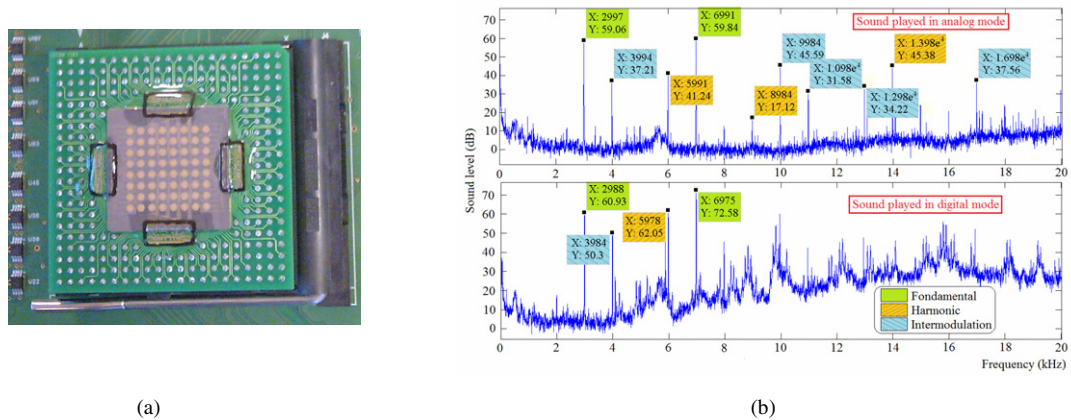
Fig. 4. (a) A digital loudspeaker connected on the driving electronic board; (b) Recordings of the same reference signal played in an analog and digital approach (clock frequency = 44.1 kHz).
