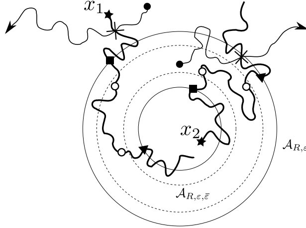
Figure 3: In this picture the points marked with \star are x_i , i = 1, 2 . The symbols \blacksquare, \blacktriangle refer to the times \sigma^{\text{in}} and \sigma^{\text{out}} , respectively. The symbol \circ represents the times \sigma^{\text{in}} + \delta and \sigma^{\text{out}} - \delta , respectively. Finally, the symbol \times indicates that Condition (5.22) is fulfilled.
