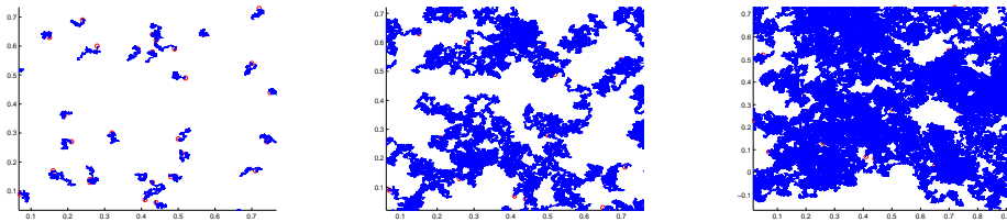
Figure 1: Simulations of \mathcal{O}_t in the case d = 2 , at small, intermediate, and large times.
