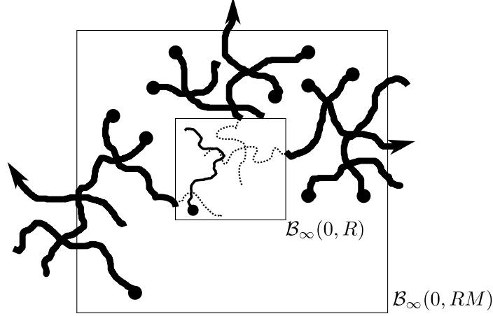
Figure 2: The plot represents a configuration in E_{R,M}(0) with K = 3 , see (5.6)-(5.7). The thick lines belong to the branches. The symbol \blacktriangleright indicates a connection to infinity.
