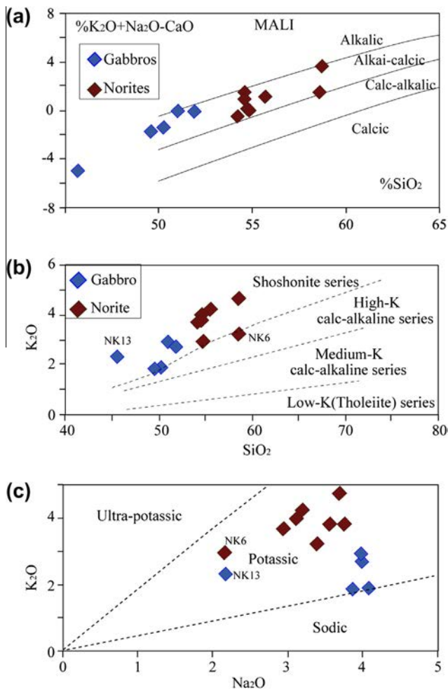
Fig. 6. (a) MALI diagram from Frost et al. (2001). Plot of Na_2O + K_2O - CaO vs SiO_2 showing the alkali-calcic feature of the Kekem rocks, (b) K_2O vs SiO_2 diagram after Peccerillo and Taylor (1976), shows the shoshonitic affinity of gabbro-norites from Kekem and (c) K_2O vs Na_2O confirms the high-k feature of gabbro-norites from Kekem.
