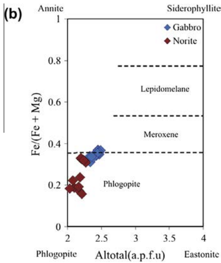
Fig. 5b. Classification of micas of the gabbro-norites from Kekem.
