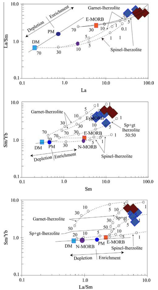
Fig. 12. REE variations in gabbro-norites of Kekem, (a) La vs La/Sm, (b) Sm/Yb vs Sm and (c) Sm/Yb vs La/Sm. Mantle array defined by depleted MORB mantle (DM; McKenzie and O’Nions, 1991) and primitive mantle (PM, Sun and McDonough, 1989) compositions. Melting curves for spinel-lherzolite and garnet-lherzolite sources with both DM and PM compositions after Aldanmaz et al. (2000); circled dots on each melting curve correspond to degrees of partial melting for a given mantle source. Also shown are N-MORB and E-MORB compositions of Sun and McDonough (1989).
