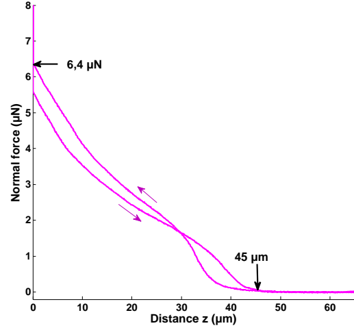
Fig. 11. Force-distance curves on functionalised PPy in \text{LiClO}_4 salt by electropolymerisation in liquid medium (pH 10, spring constant 0.3\ \text{N/m} ).
