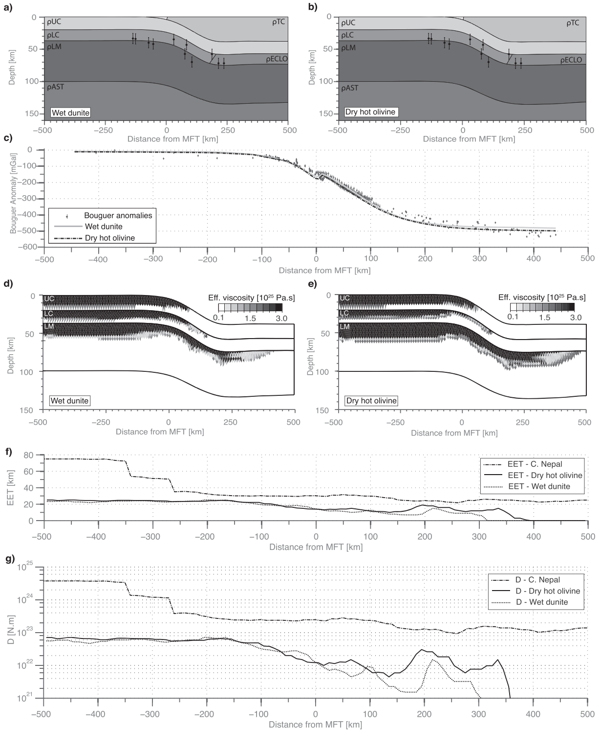
Figure 3. Preferred model results. (a, b) Resulting geometry with projected seismic Moho depths (dots with error bars) and density structure. Densities as in Table S1 and \rho_{ECLD} = 3050 \text{ kg m}^{-3} . (c) Synthetic (lines) and observed Bouguer anomalies (dots with error bars). (d, e) Effective viscosity profiles. (f, g) Effective elastic thickness and flexural rigidity of the preferred models and of the Nepali model (Berthet et al., submitted manuscript, 2013) for comparison.
