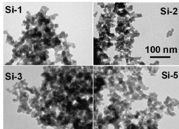
Fig. 9 TEM imaging of isolated silica Si-1 , Si-2 , Si-3 and Si-5 .
