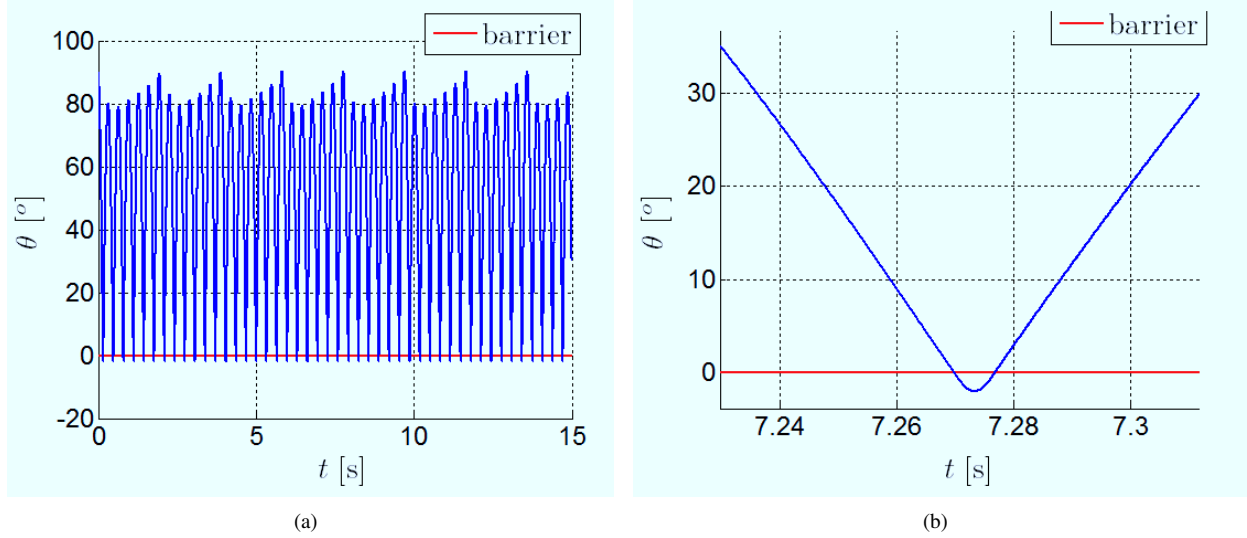
Figure 5. Coupled motor-cart-pendulum-barrier system with gap/l_p = 0 : (a) pendulum displacement over time and initial position of the barrier (b) zoom of an impact.
