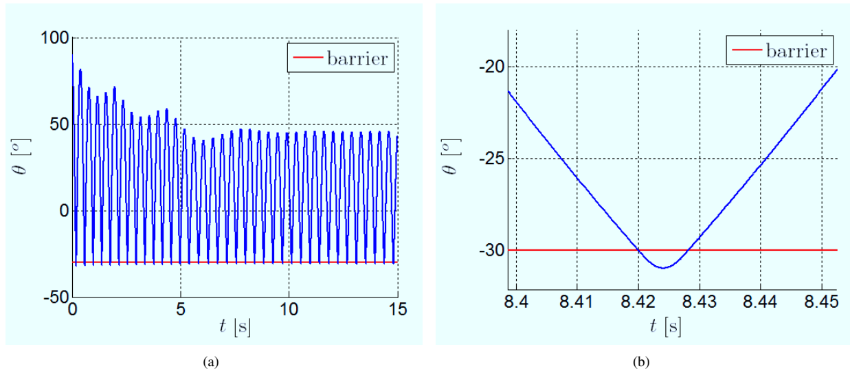
Figure 7. Coupled motor-cart-pendulum-barrier system with gap/l_p = 0.5 : (a) pendulum displacement over time and initial position of the barrier and (b) zoom of an impact.
