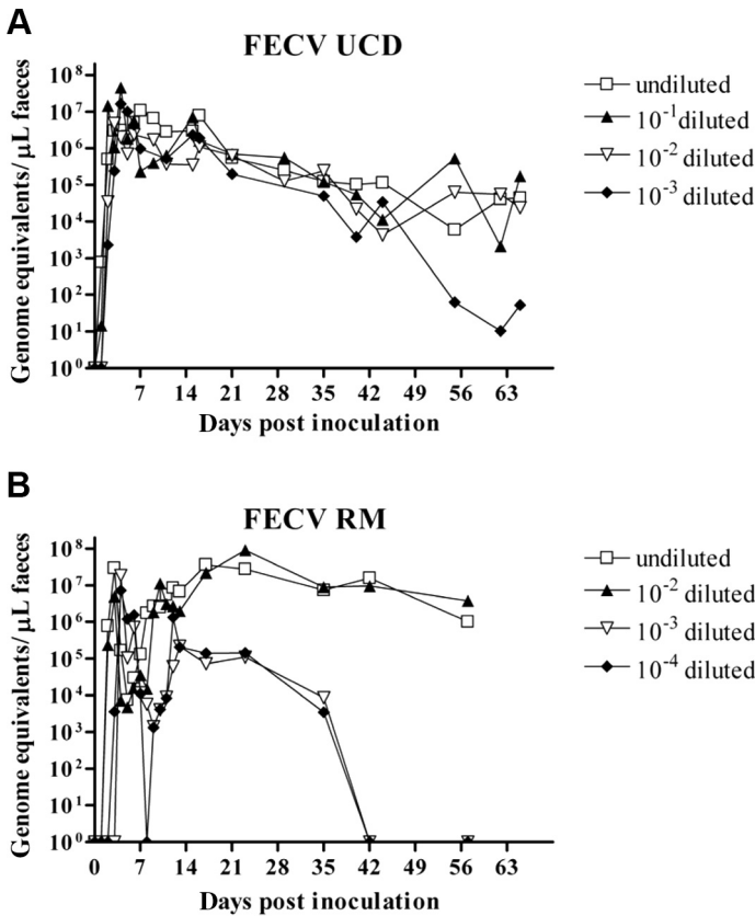
Figure 1. Faecal shedding of virus by cats included in infection experiments A2 and B2 after inoculation with FECV UCD (A) or FECV RM (B), as monitored by TaqMan ® RT-PCR. Means per group ( n = 2). Note that RNA quantities below 3 \times 10^3 cannot be considered accurate (real quantities are probably lower) due to the non-linear relationship between input RNA and Ct value in the assay in the lower concentration range.
