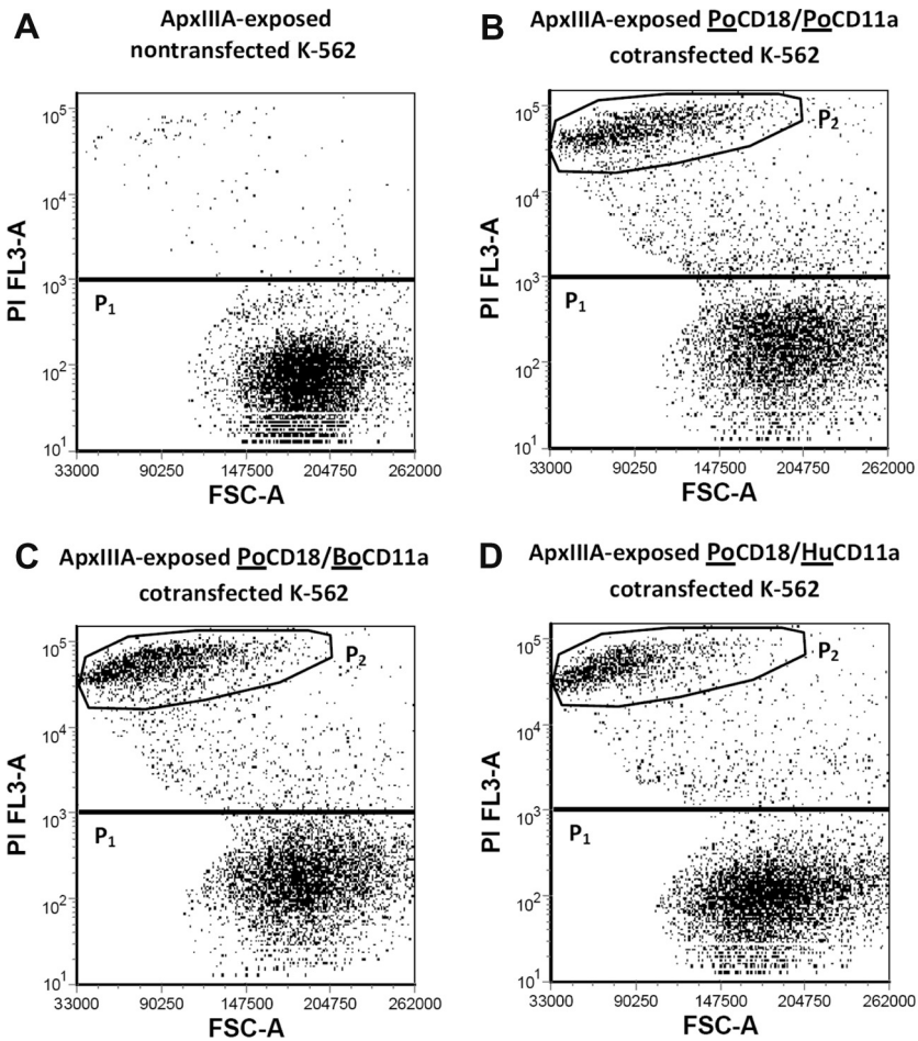
Figure 2. K-562 cells accumulate PI upon ApxIIIa exposition when expressing porcine CD18-containing LFA-1s. PI versus forward scatter (FSC) dot plot from flow cytometric analysis of ApxIIIa-exposed control (top, left) and double transfected K-562 cells. Only the P2 populations expressed the intended LFA-1.
