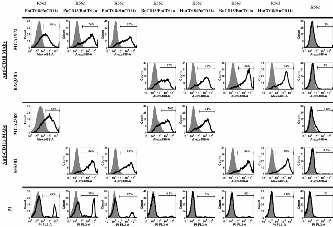
Figure 1. Flow cytometric phenotyping of nontransfected (last column on the right) and double transfected K-562 cells. Ectopic LFA-1 cell-surface expression was probed by detection of cell-surface expression of either the CD18 (rows 1–2) or the CD11a (3–4) subunit. Distributions of control and principal single cell fluorescence intensities were obtained after using an isotype-matched non pertinent (filled, grey) or an anti-CD18 or -CD11a primary antibody (open, white) respectively, before detection with Alexa Fluor 488-conjugated secondary Abs. Cells undergoing cell death were defined as those showing PI incorporation (row 5) and their relative proportion was established in mock- (unimodal grey distribution) and ApxIIIa-exposed (uni- or bimodal white) non- or cotransfected K-562 cells. Range of Alexa 488/PI positivity is given in each panel along with percentage of positive cells. See text for details.
