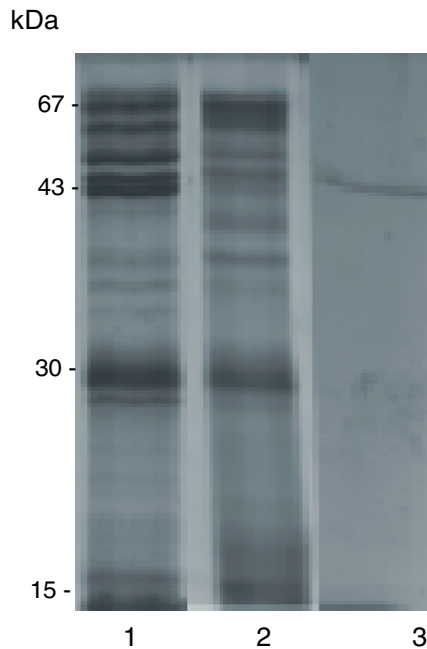
Figure 1. Silver-stained 1D SDS-PAGE gel (15%) analysis of ES products (5 µg, lane 1), 1st unbound fraction (1.25 µg, lane 2) and cystatin-binding fraction (0.5 µg, lane 3). Molecular markers are indicated on the left (in kDa).
