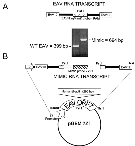
Figure 1. A schematic diagram of the artificial EAV TaqMan ® mimic RNA construct. RNA was prepared by in-vitro transcription using T7 RNA polymerase. The EAV TaqMan ® probe site (⋯⋯⋯) was disrupted in the mimic by the insertion of a 295 bp fragment of human \beta -actin and was detected by a second probe (▨▨▨▨). The location of PCR primers (EAV10 and EAV12) are shown.
